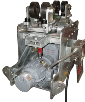
T-200-AT EXTRA HEAVY DUTY ARTICULATING TRACTOR
