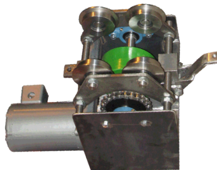
TRACTOR WITH MANUAL TENSION RELEASE ARM
